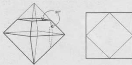
Fig. 6-40. Looking at the face (right) created by truncating all 6 points of an octahedron (left, shown with only one point truncated and another at 90^\circ ).
