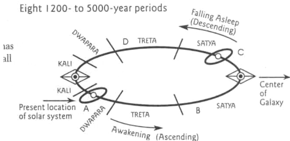
Fig. 4-6. The cycle of the precession of the equinoxes; A is the point of pole shift.
