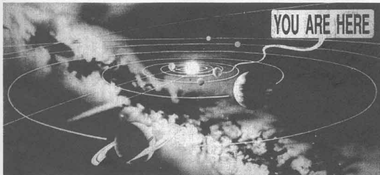
Fig. 2-33. Earth's location in the solar system.
