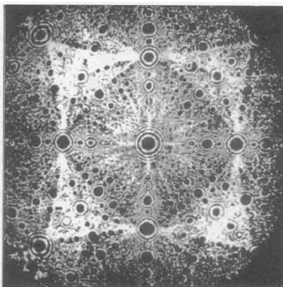
Fig. 6-29. Atomic pattern of a crystal matrix.
