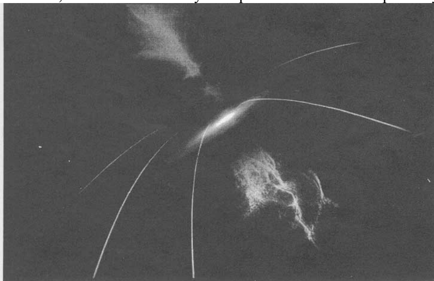
Fig. 2-34. Quasar (quasi-stellar radio source) believed to be the most distant and luminous objects in the universe.
