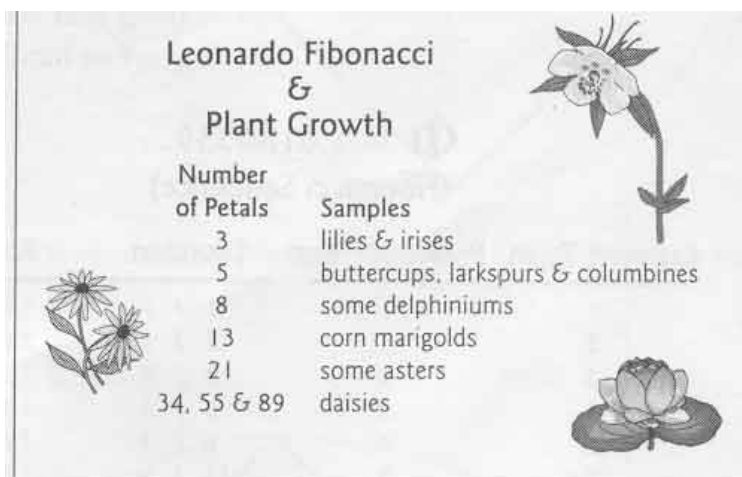
Fig. 8-1. Fibonacci sequence in plant growth.
