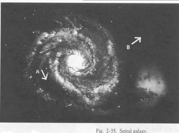
Fig. 2-35. Spiral galaxy.
