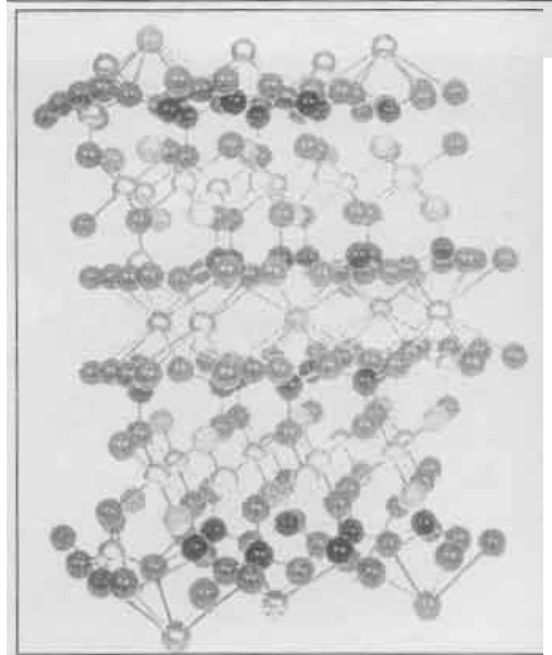
Fig. 6-33. Complex molecular formation.
