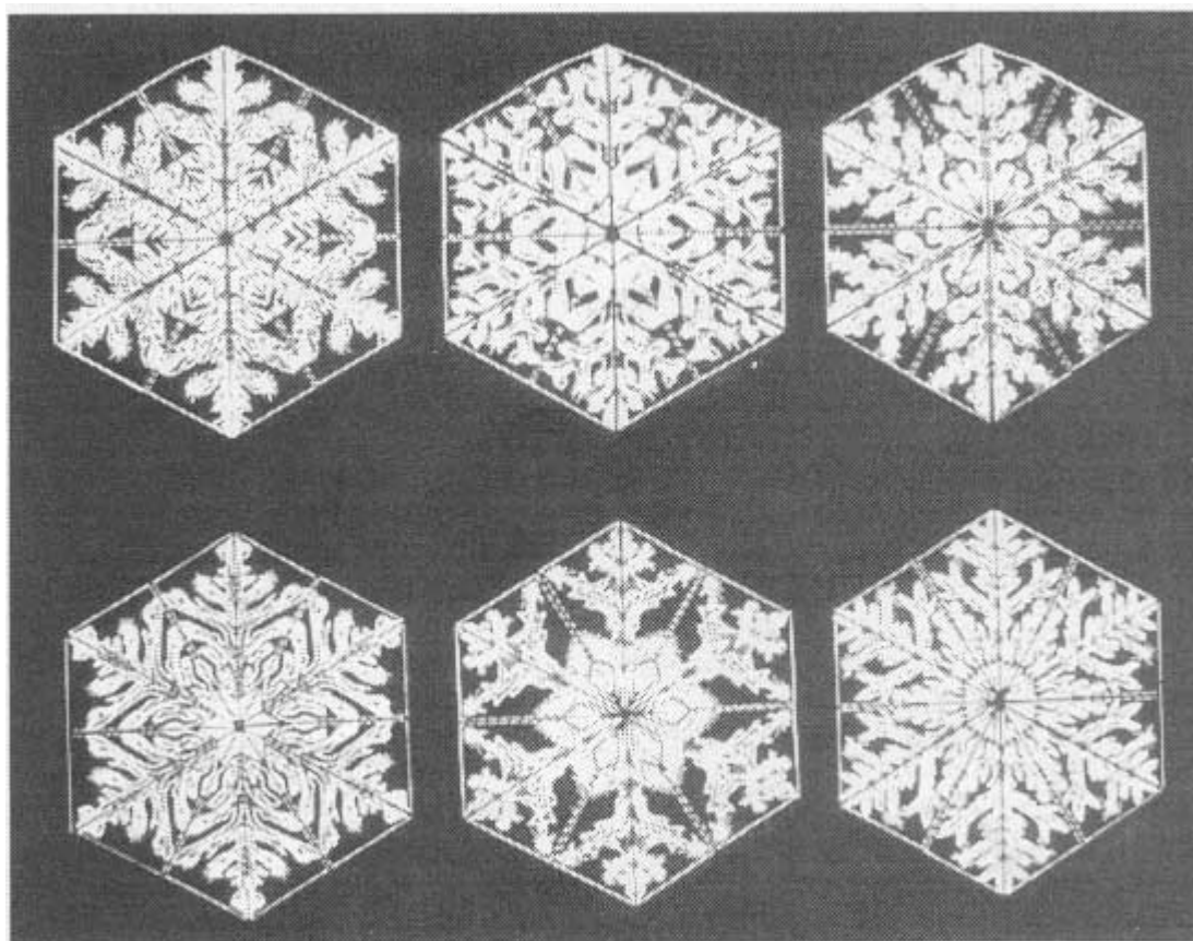
Fig. 6-46. Ice crystals, or snowflakes.
