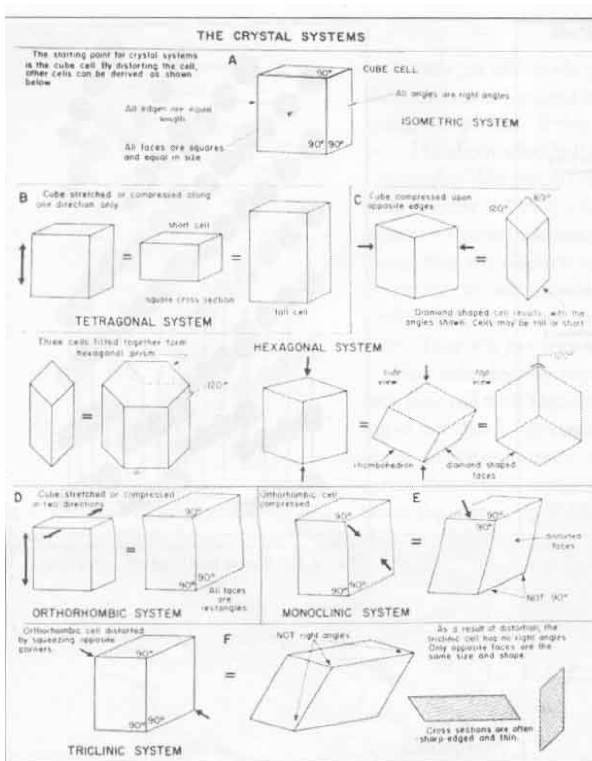
Fig. 6-34. Crystal systems.
