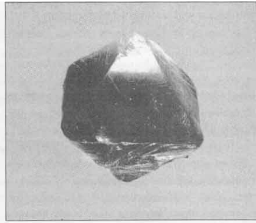
Fig. 6-35b. Fluorite crystal with an octahedral structure.
