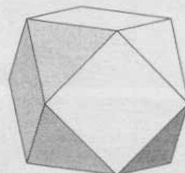
Fig. 6-41. Views of a vector equilibrium (cuboctahedron).
