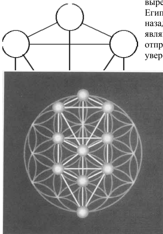
Fig. 2-23, Superimposed Tree and Seed of Life.
