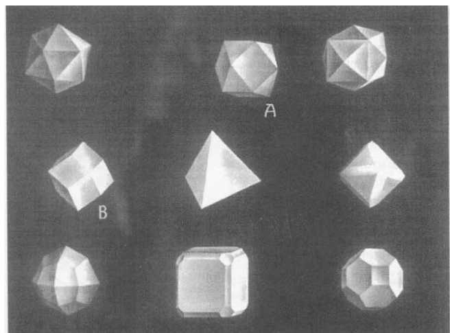
Fig. 6-43. A variety of polyhedrons. A is a cuboctahedron and B is a rhombic dodecahedron.
