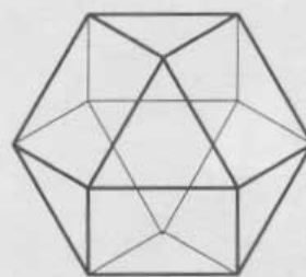
Fig. 6-40. Looking at the face (right) created by truncating all 6 points of an octahedron (left, shown with only one point truncated and another at 90^\circ ).
