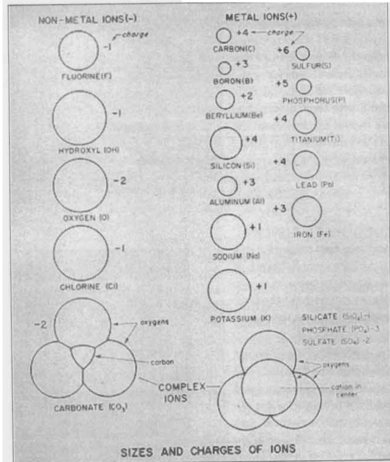
Fig. 6-30. Sizes and charges of ions.
