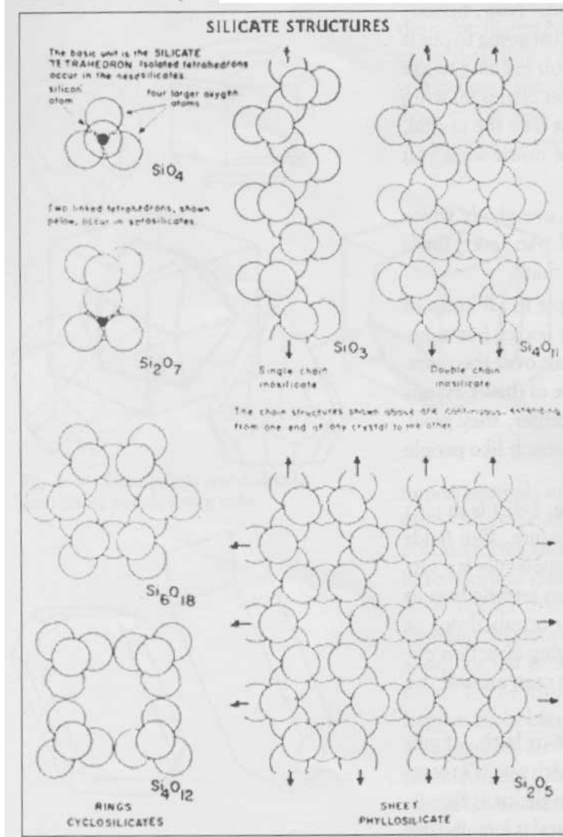
Fig. 6-49. Silicon makes forms and relationships.
