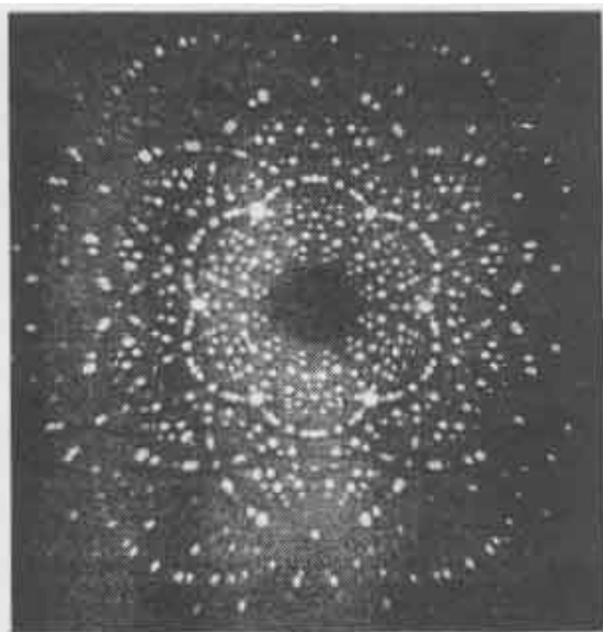
Fig. 6-28. Atomic pattern of a beryl crystal.
