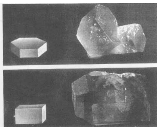
Fig. 6-44. Comparing atoms and crystals, hexagonal (beryl) and orthorhombic (topaz) systems.
