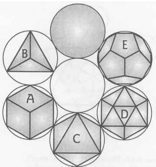
Fig. 6-15. The five Platonic solids.
