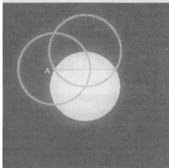
Fig. 5-36. Third sphere, second motion/day of Genesis. When sitting in the center of the uppermost circle/sphere and looking down, the horizontal line is seen as a circle.
